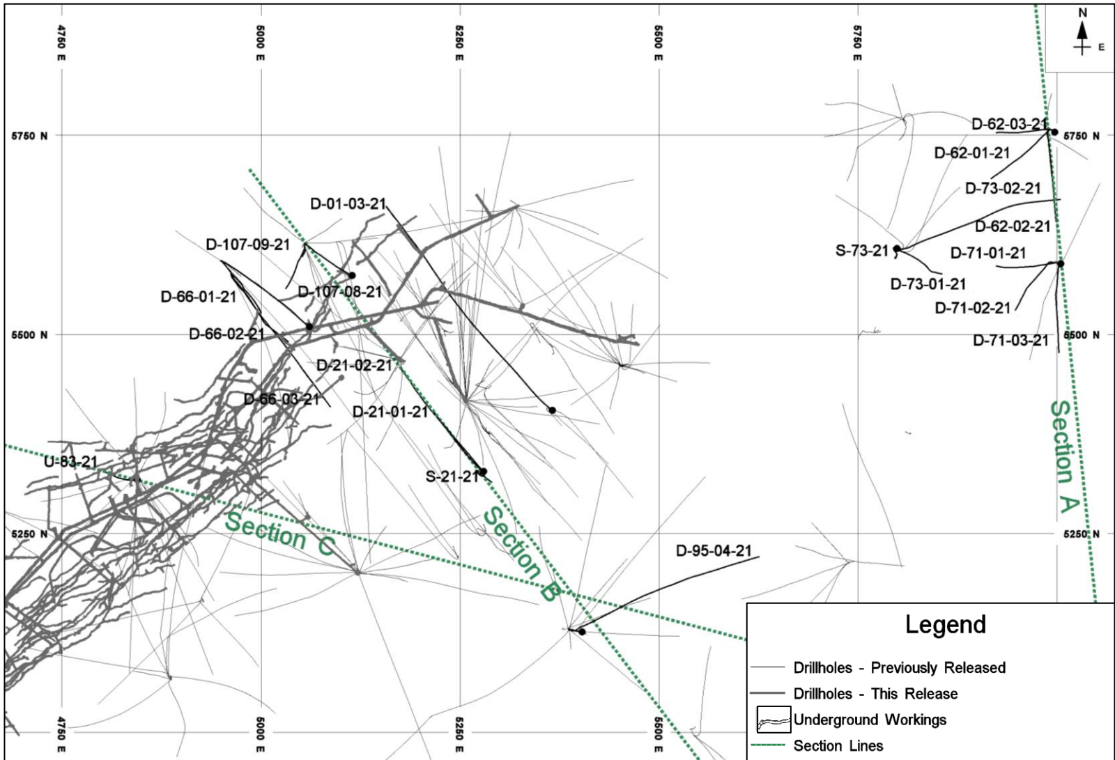
Figure 1 – Plan view of drill hole and section line locations
