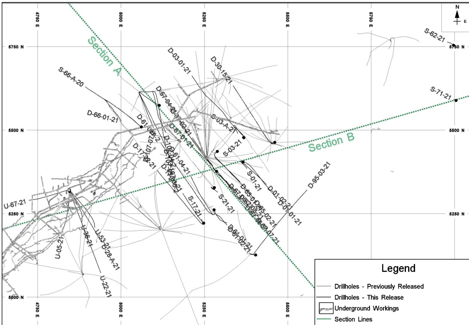
Figure 1 – Plan view of drill hole and section line locations
