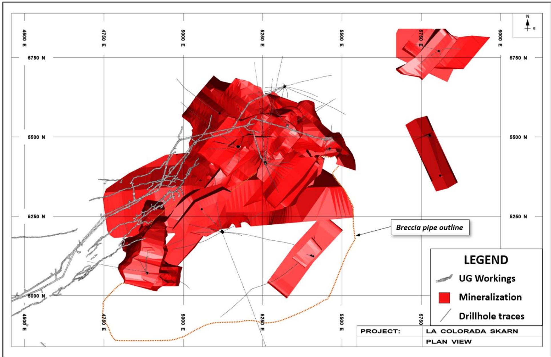
Figure 4 – Plan view of skarn bodies
