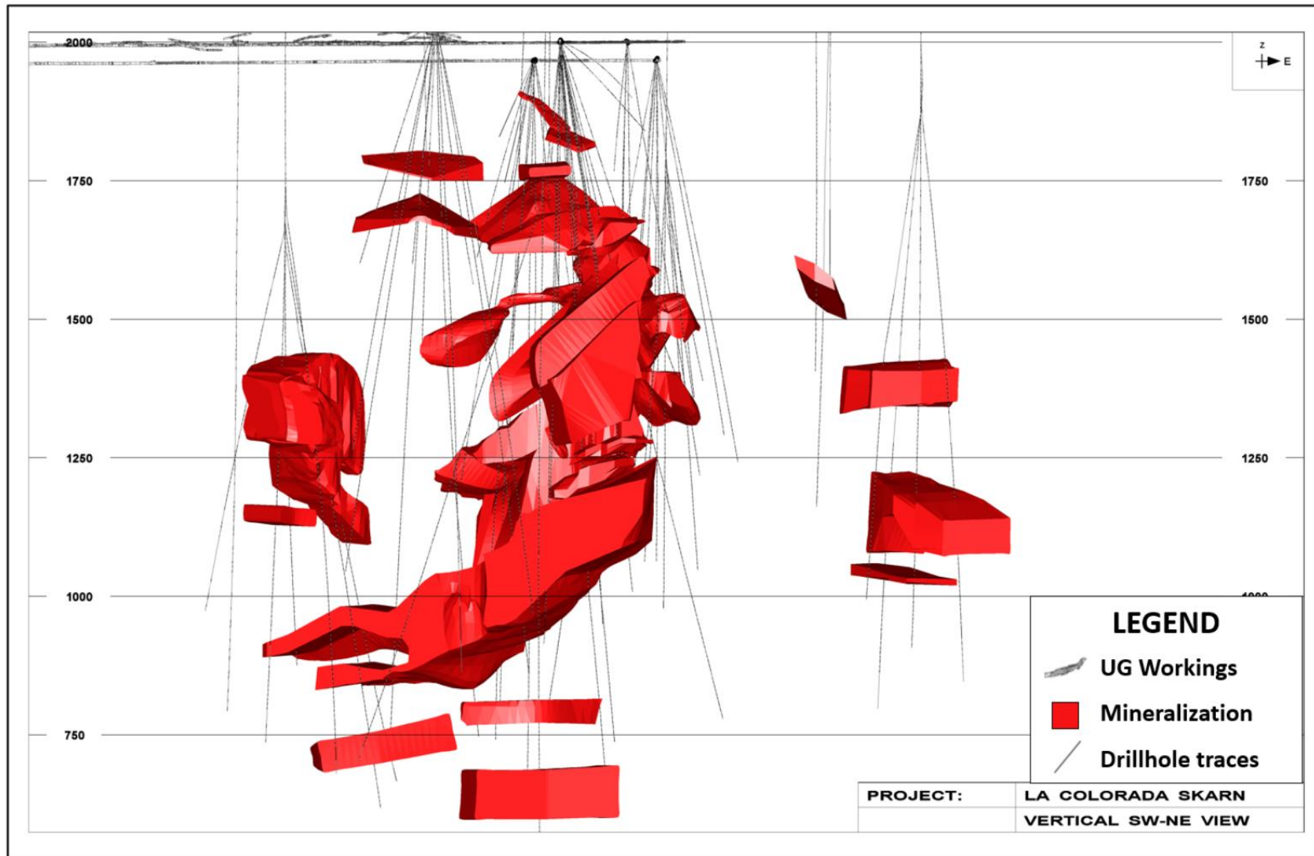
Figure 5 – Sectional view of skarn bodies (View to NW)
