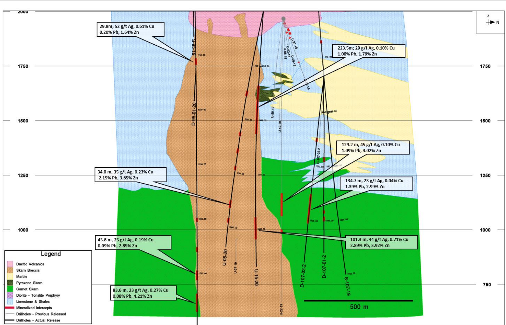
Figure 2 – Cross Section A
