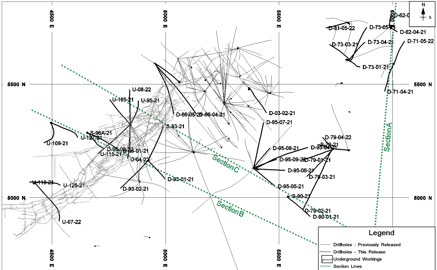
Figure 1 – Plan view of drill hole and section line locations
