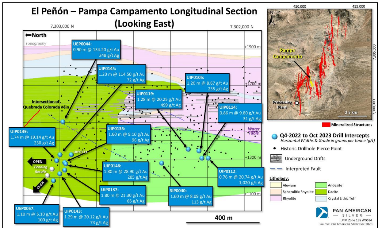
Figure 2. El Peñon – Pampa Campamento Long Section
