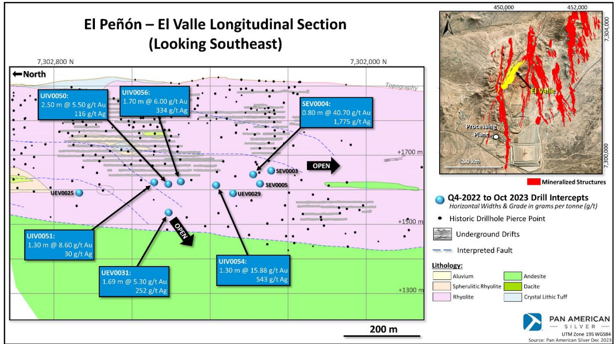
Figure 1. El Peñon - El Valle Long Section
